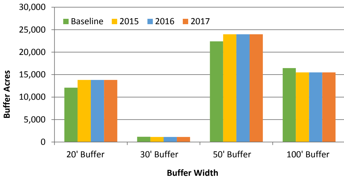
Figure 2. Nitrogen Reducing Buffers Installed on Croplands from CY2015 through CY2017, compared to Baseline (CY2006), Falls Lake Watershed*
