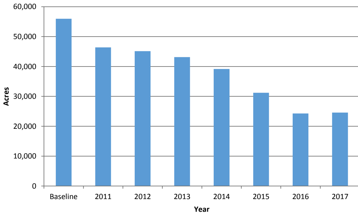
Figure 5. Total Reported Cropland Acres in the Falls Lake Watershed, Baseline (2006), 2011-2017
