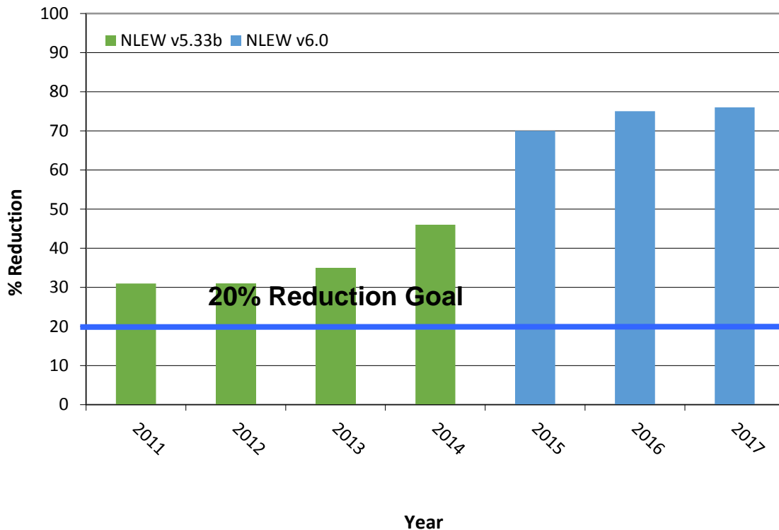
Figure 1. Collective Nitrogen Loss Reduction Percent 2011 to 2017, Falls Lake Watershed.
