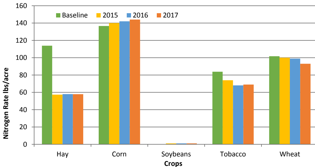
Figure 3. Average annual nitrogen fertilization rate (lb/ac) for agricultural crops for the baseline (2006), 2015-2017, Falls Lake Watershed
