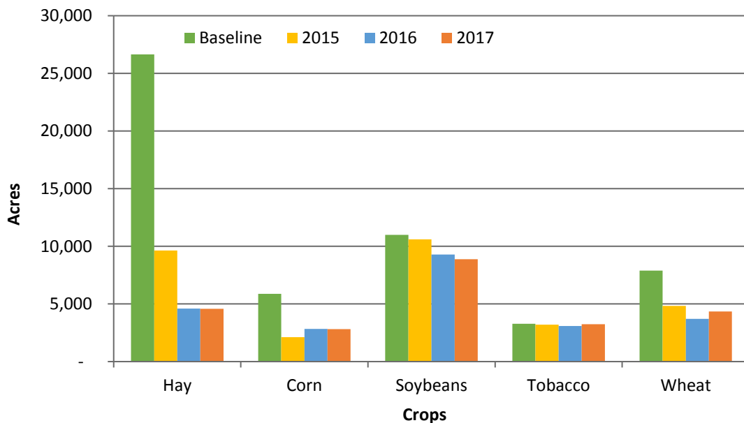
Figure 4. Reported Acreage of Major Crops for the Baseline (2006), 2015-2017, Falls Lake Watershed
